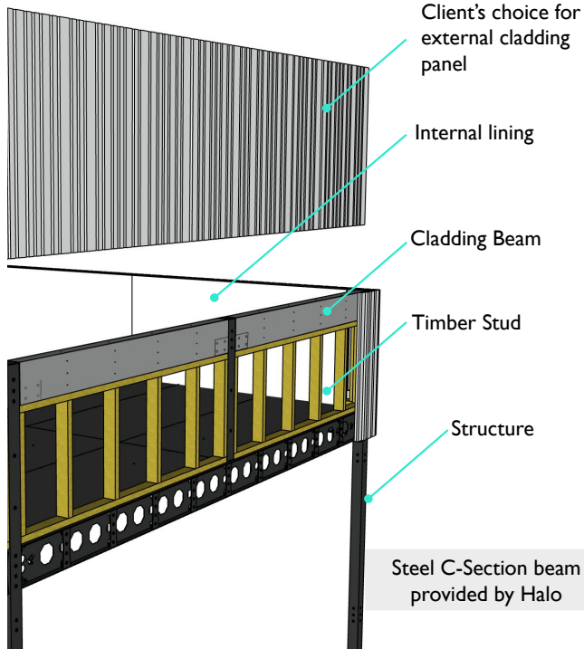
EXAMPLE CLADDING BUILD UP
