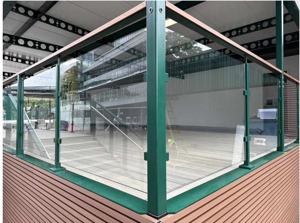
EXAMPLE TOUGHENED GLASS HANDRAIL WITH POWDER COATED GREEN STEEL AND HARDWOOD SAPELE HANDRAIL
