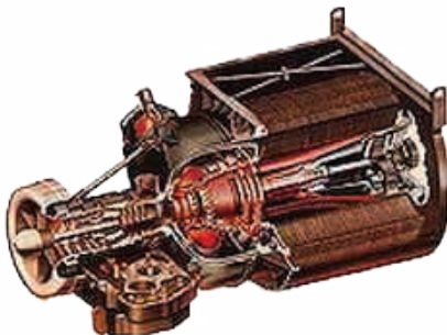
AGT-1500 Gas Turbine
