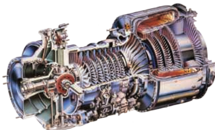
T-55 Turboshaft
