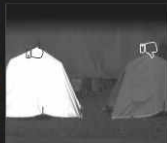
ULTRA VIOLET (250-380 nm)
